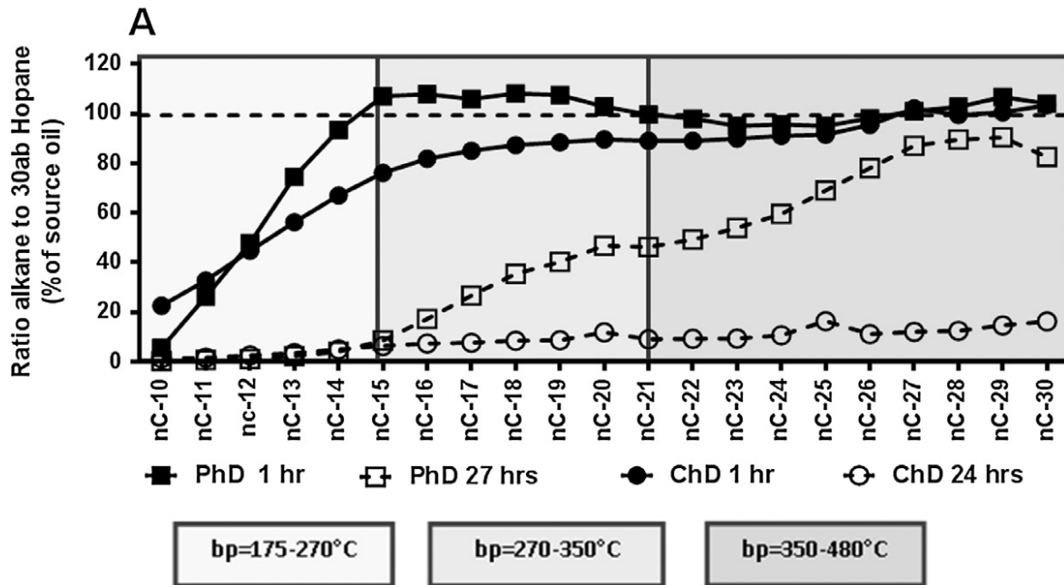
Figure 29 Biodegradation rates of physically dispersed versus chemically dispersed Macondo Oil based on laboratory plume studies conducted by SINTEF. (Brakstad et al., 2014)
