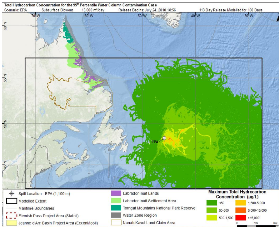
Figure 23. Maximum total hydrocarbon concentration (THC) at any depth in the water column for the 95 th percentile water column contamination case from a subsurface blowout.
