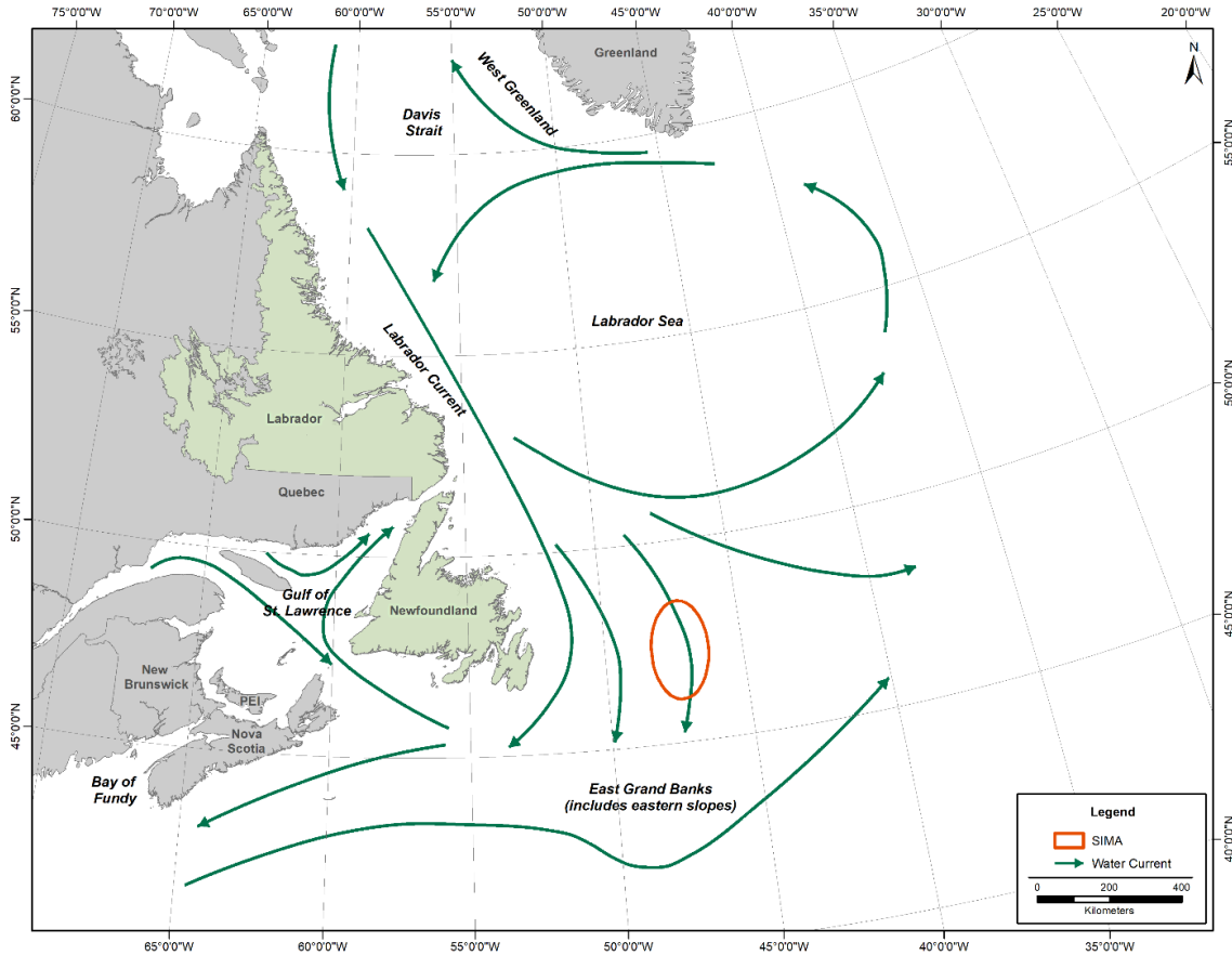
Figure 6 Overview of ocean currents in the RSA. (Equinor Canada)
