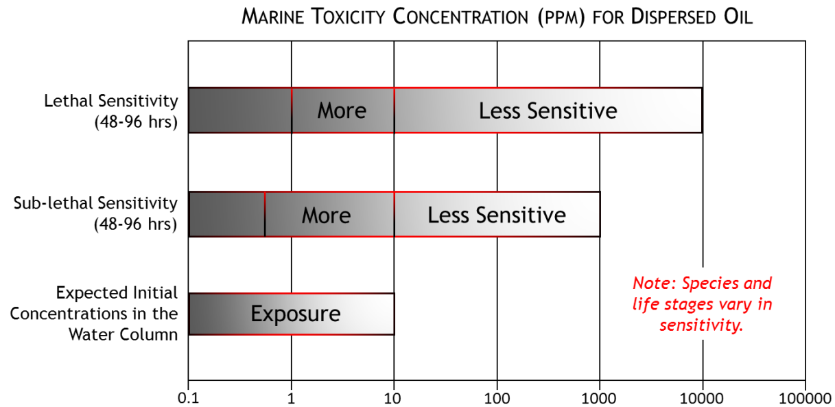
Figure 26 Sensitivity thresholds to dispersed oil concentrations. (Developed from data reviewed in NRC, 1989; NRC, 2003; and NRC, 2005)
