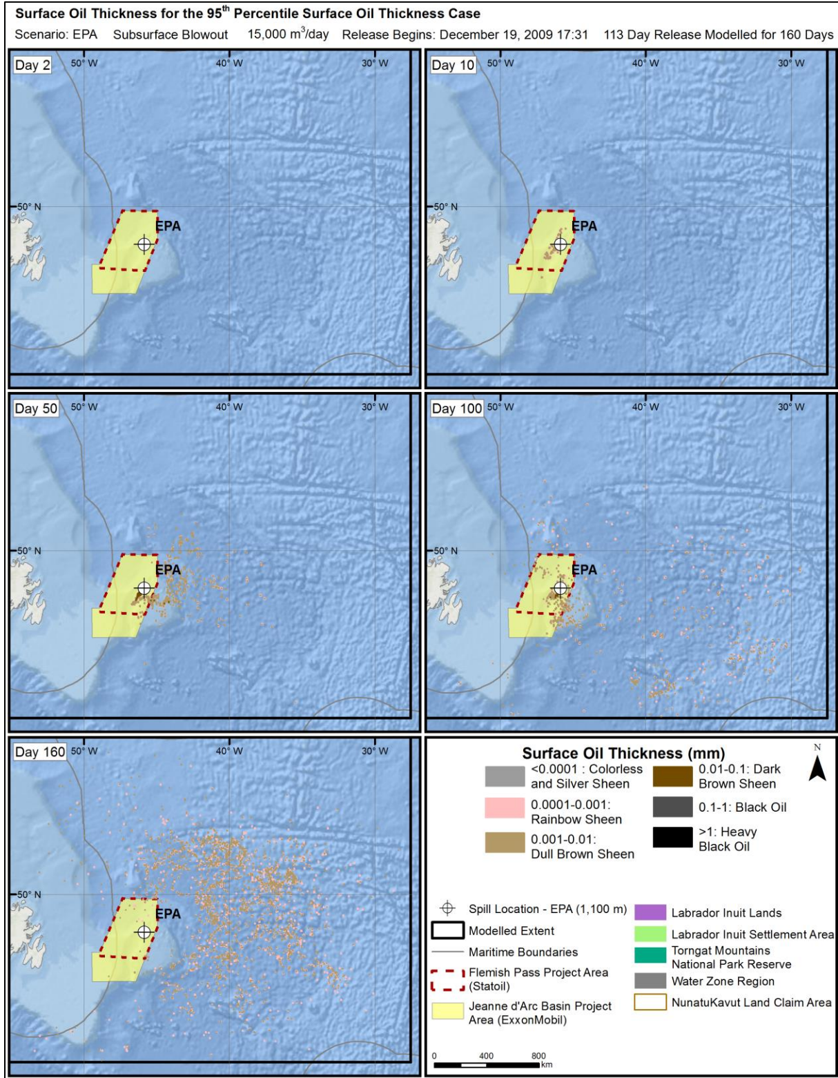
Figure 20 Predicted surface oil thickness for the 95th percentile surface oil exposure case at days 2, 10, 50, 100, and 160.
