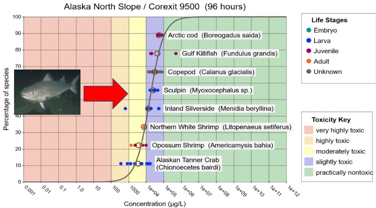
Figure 27 Species sensitivity distribution comparing a deep sea species (sablefish) to other organisms LC50s when exposed to ANS dispersed oil. (Naile, 2016)
