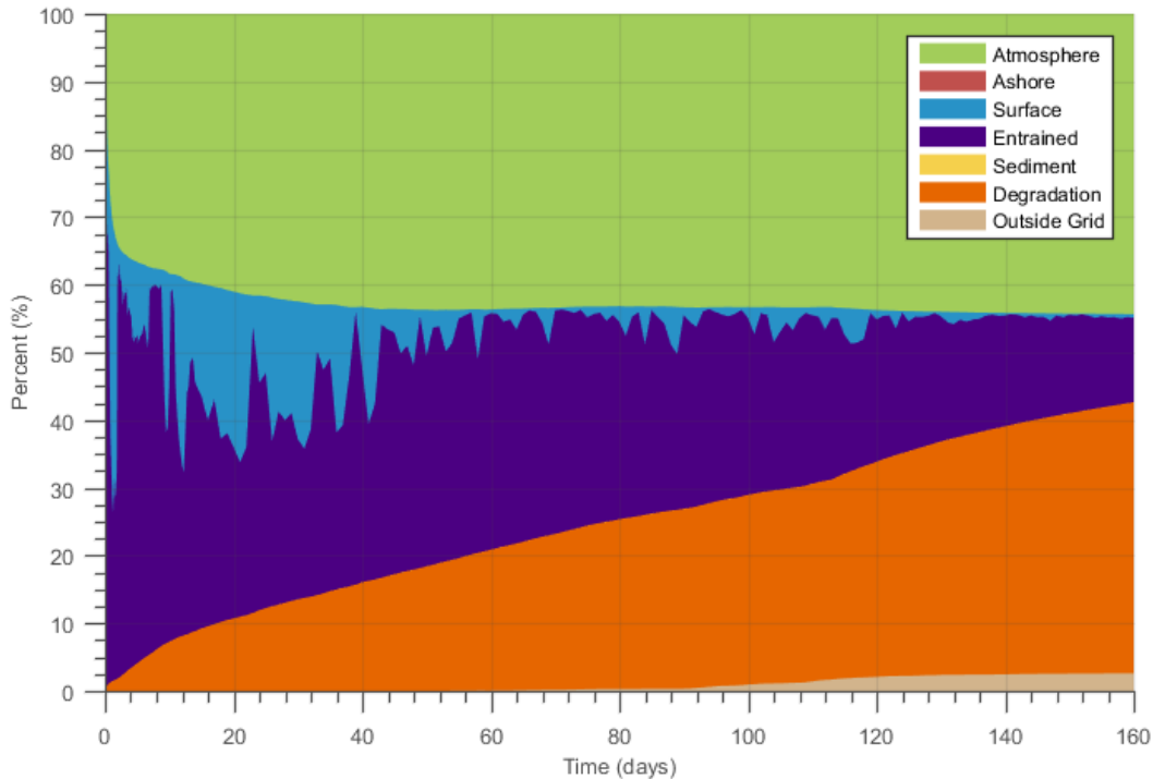
Figure 21. Mass balance plots for the 95 th percentile surface oil thickness case.
