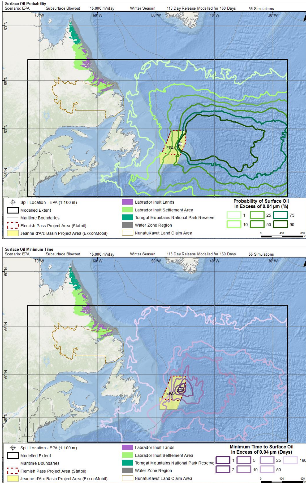
Figure 18 Winter probability of average surface oil thickness > 0.04 µm (top) and minimum time to threshold exceedance (bottom) resulting from a subsurface blowout.
