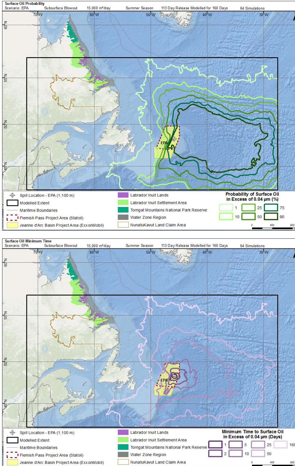
Figure 17 Summer probability of average surface oil thickness > 0.04 µm (top) and minimum time to threshold exceedance (bottom) resulting from a subsurface blowout.
