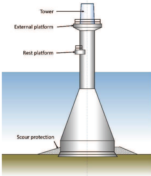
Gravity base
