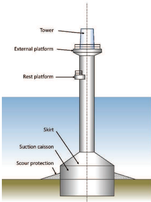
Suction bucket
