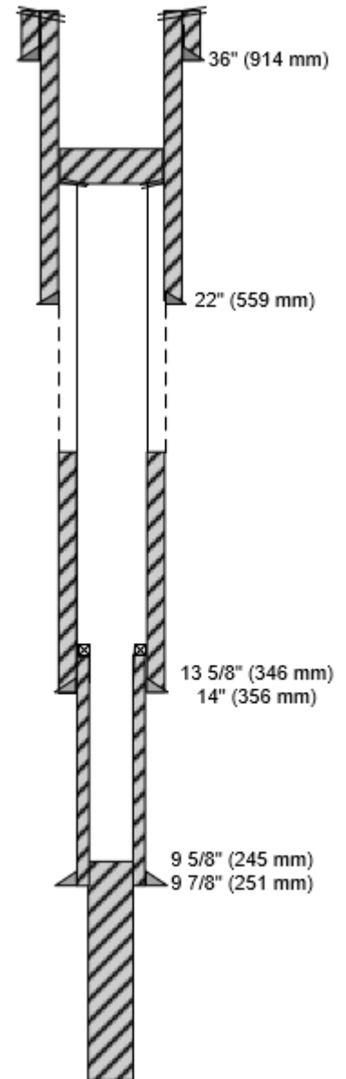
Figure 3: Well Abandonment Example
