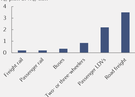
Global average energy use in 2010
