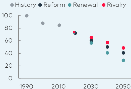
Energy intensity by scenario Index, 1990=100
