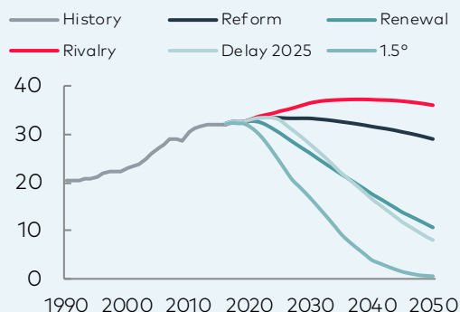
Global CO 2 emissions by scenario and sensitivity Gt
