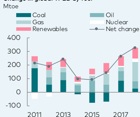
Change in global TPED by fuel
