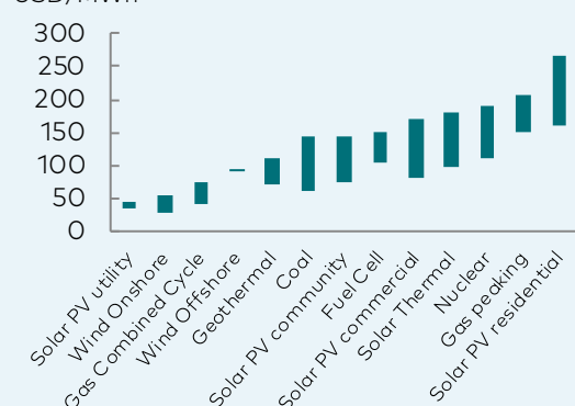
LCOE ranges in US, unsubsidised basis USD/MWh
