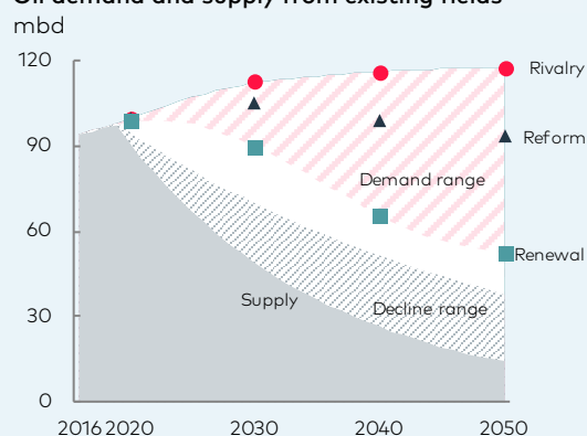
Oil demand and supply from existing fields
