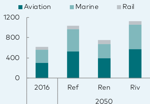
Global non-road transport by mode and scenario Mtoe
