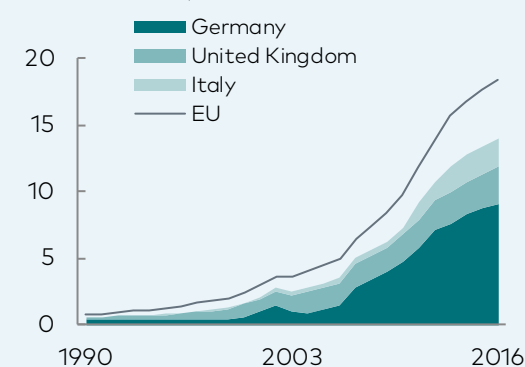
EU biogas production Bcm, methane equivalent
