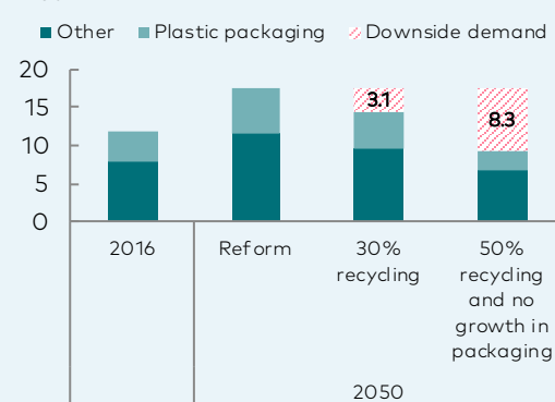
Petrochemical oil demand sensitivities in Reform mbd
