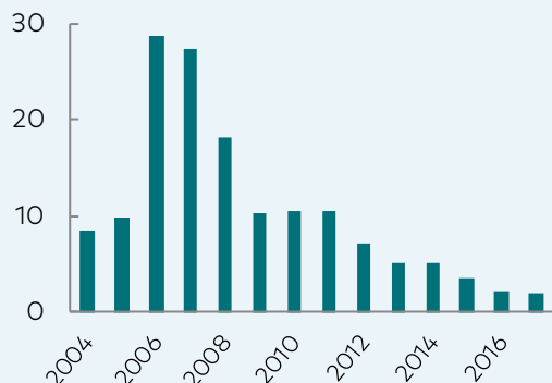
Annual global investments in biofuels supply Bn USD
