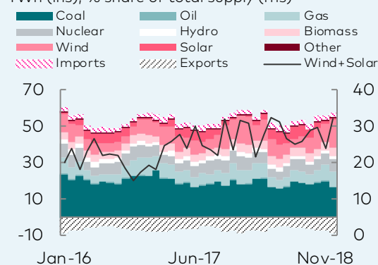
Germany's electricity generation and supply TWh (lhs), % share of total supply (rhs)
