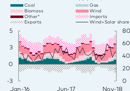
Denmark's electricity generation and supply TWh (lhs), % share of total supply (rhs)
