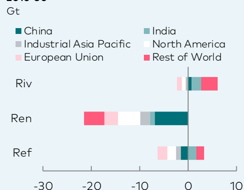
Change in CO 2 emissions by region and scenario, 2016-50
