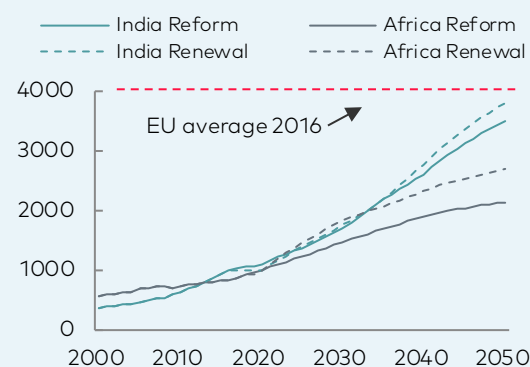
Electricity demand per household
