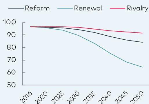
Oil share of non-road transport %
