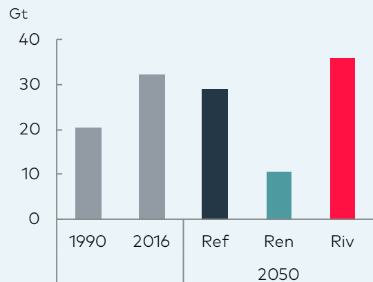
Annual net energy-related CO 2 emissions by scenario
