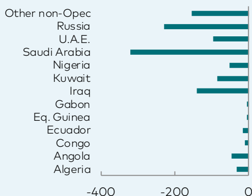
Opec+ supply cuts to be implemented by 1H 2019 kbd
