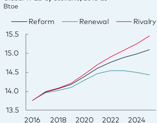
Global TPED by scenario, 2016-25
