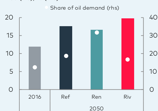
Petrochemical oil demand by scenario mbd (lhs), % (rhs)
