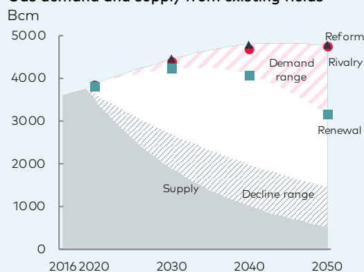
Gas demand and supply from existing fields
