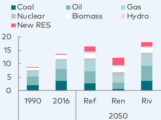
Global TPED by fuel and scenario Btoe
