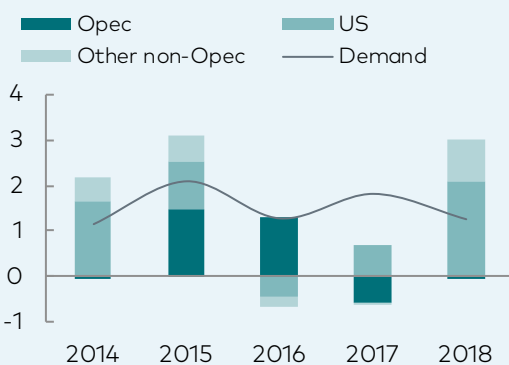
Annual change in global oil balance mbd
