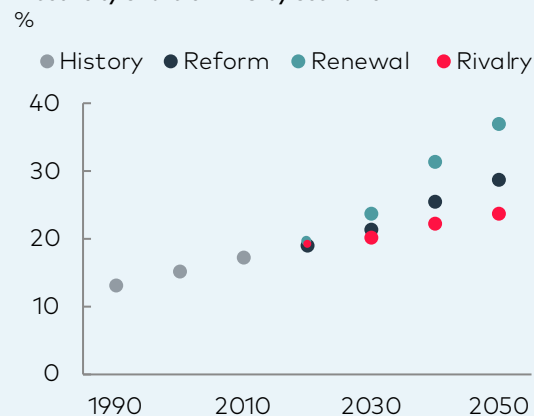
Electricity share of TFC by scenario
