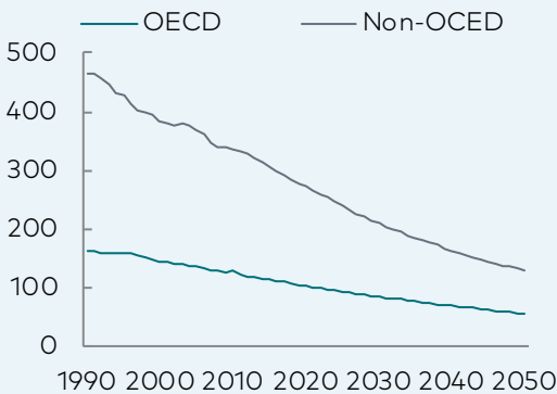
Energy intensity development in Reform Toe/million USD (Real 2010 USD)
