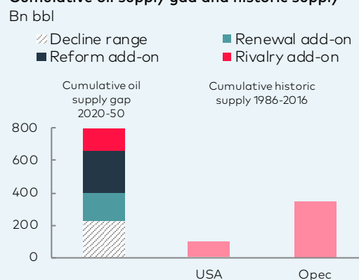
Cumulative oil supply gap and historic supply
