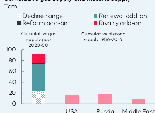
Cumulative gas supply and historic supply
