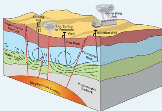
Diagram of a geothermal power plant
